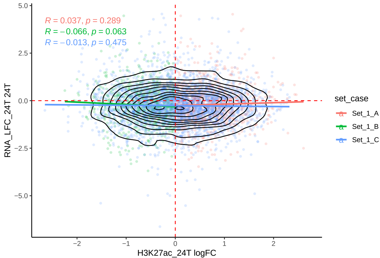
LTR_summit H3K27ac_24T and RNA LFC at 24T set_1
